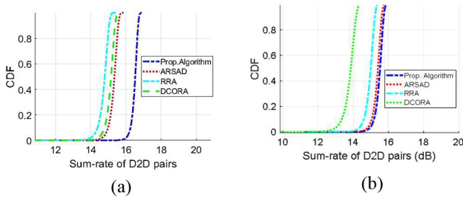
Fig. 5. Cumulative distribution of D2D sum rate with three other approaches when (a) Z = 20 and N = 10 , (b) Z = 20 and N = 20 and P_{2\max}^d = P_{\max}^c = 23 dBm.
