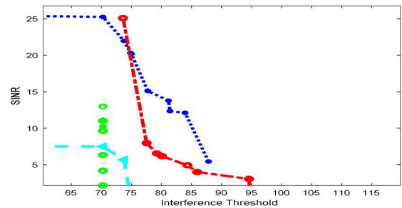
Fig. 13. SINR against the interference threshold of the proposed algorithm with three other approaches when Z = 20 and N = 10 , and P_{2\max}^d = P_{\max}^c = 23 dBm.
