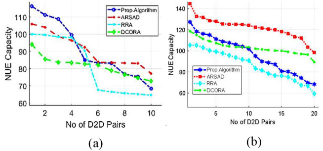
Fig. 7. NUE's capacity against the number of D2D pairs with three other approaches when (a) Z = 20 and N = 10 and (b) Z = 20 and N = 20 and P_{2\max}^d = P_{\max}^c = 23 dBm.
