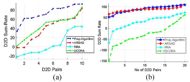
Fig. 6. D2D pair's sum rate against the number of D2D pairs for the different approaches when (a) Z = 20 and N = 10 , (b) Z = 20 and N = 20 and P_{2\max}^d = P_{\max}^c = 23 dBm.
