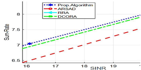
Fig. 12. Sum rate against the SINR of the proposed algorithm with three other approaches when Z = 20 and N = 10 , and P_{2\max}^d = P_{\max}^c = 23 dBm.
