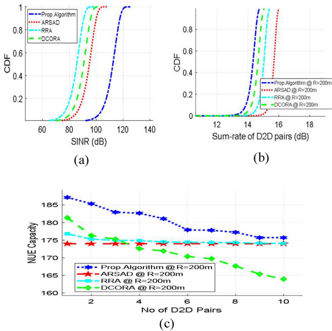
Fig. 10. (a) SINR, (b) sum rate, and (c) NUE capacity against number of D2D pairs when R = 200 m and a distance between D2D pairs = 14 m.
