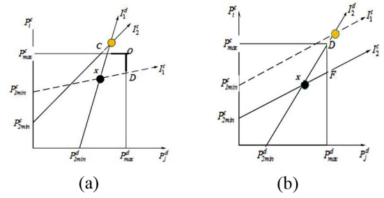
Fig. 15. Feasible region of optimal power control for NUE and D2D user based on the magnitude of the (P_{\max}^c, P_{\max}^d) . Depicts Power perspective of D2D pair (a) 1 reuse with NUEs (1 and 2), and (b) 2 reuse with NUEs (1 and 2).
