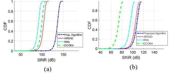
Fig. 4. SINR of D2D pairs of the proposed algorithm with three other approaches when (a) Z = 20 and \mathcal{N} = 10 , (b) Z = 20 and \mathcal{N} = 20 and P_{2\max}^d = P_{\max}^c = 23 dBm.
