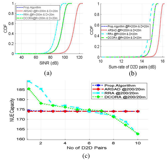
Fig. 11. (a) SINR’s CDF, (b) sum-rate’s CDF, and (c) NUE’s capacity against number of D2D pairs when R = 200 m and Max. D2D’s cluster Distance = 20 m.
