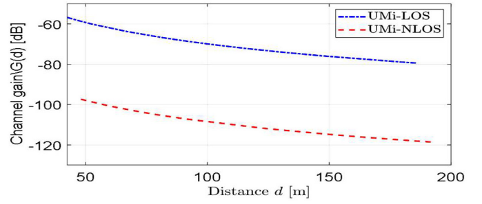
Fig. 3. Channel gain versus distance.
