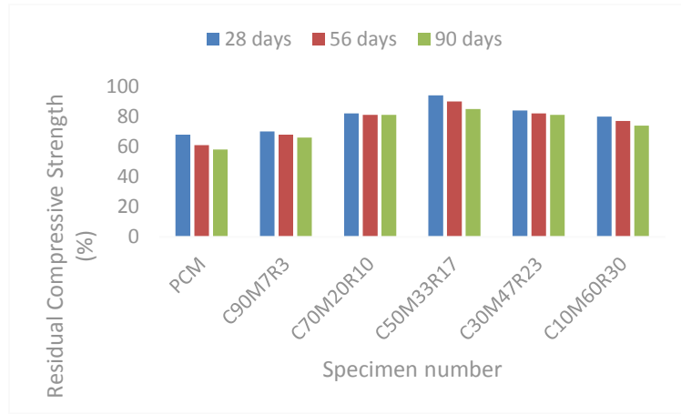
Figure 2: Strength losses as caused by H_2SO_4 attack on ternary blended GPMs
