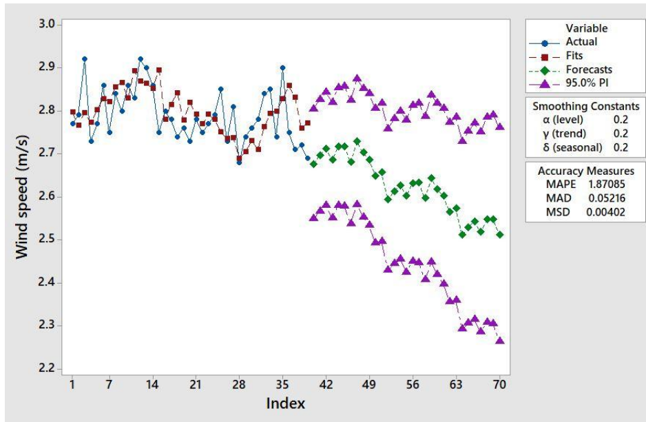
Figure 16. MINITAB Graphical Forecast when \alpha = 0.2 , \gamma = 0.2 , \delta = 0.2 of Ogun
