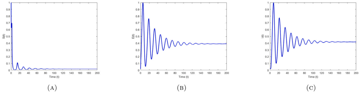
Fig. 3. Time series plot for \tau = 1.70 .
