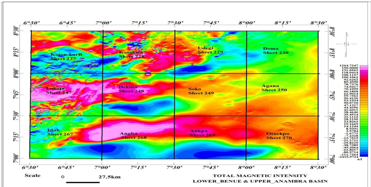
Figure 3: Total Magnetic Intensity Map of the Study Area showing major towns flown over
