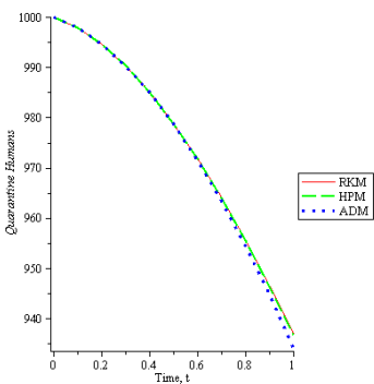
Figure 3.3: Graphical Solution of Quarantine Human Population
