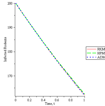
Figure 3.6: Graphical Solution of Infected Rodent Population
