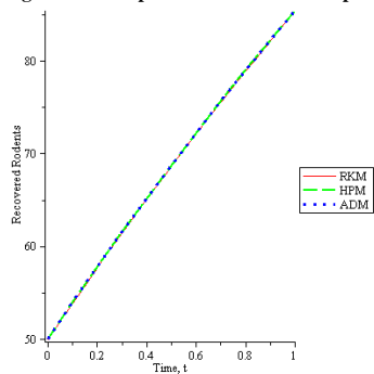
Figure 3.7: Graphical solution of Recovered Rodent Population
