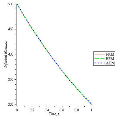
Figure 3.2: Graphical Solution of Infected Human Population
