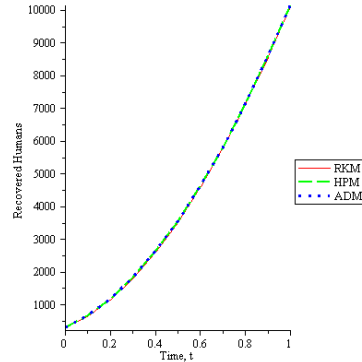
Figure 3.4: Graphical Solution of Recovered Human Population
