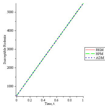
Figure 3.5: Graphical Solution of Susceptible Rodent Population
