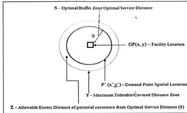
Figure 2: Formulating P-Centre algorithm.
