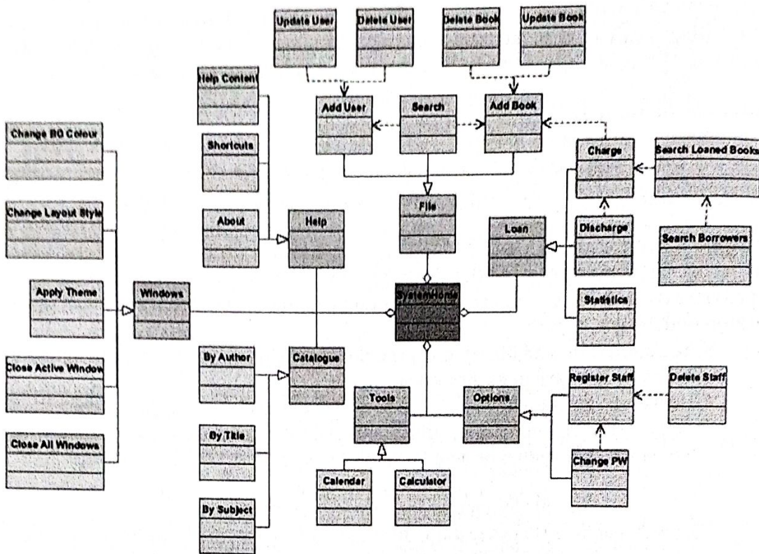
Figure 2: Class Diagram of the Developed System's User Interface
