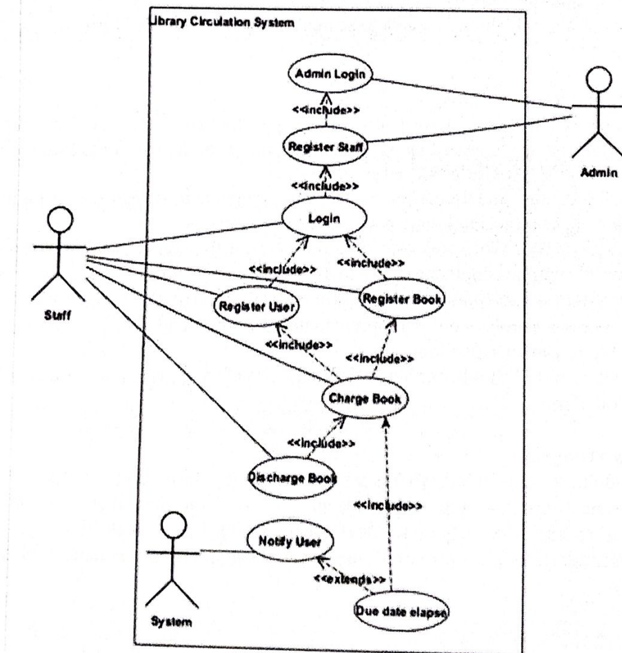
Figure 3: Use Case Diagram of the Registration Process
