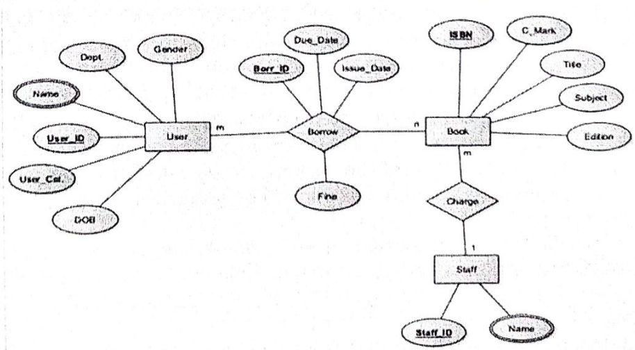
Figure 8: Entity Relationship Diagram of the Database
