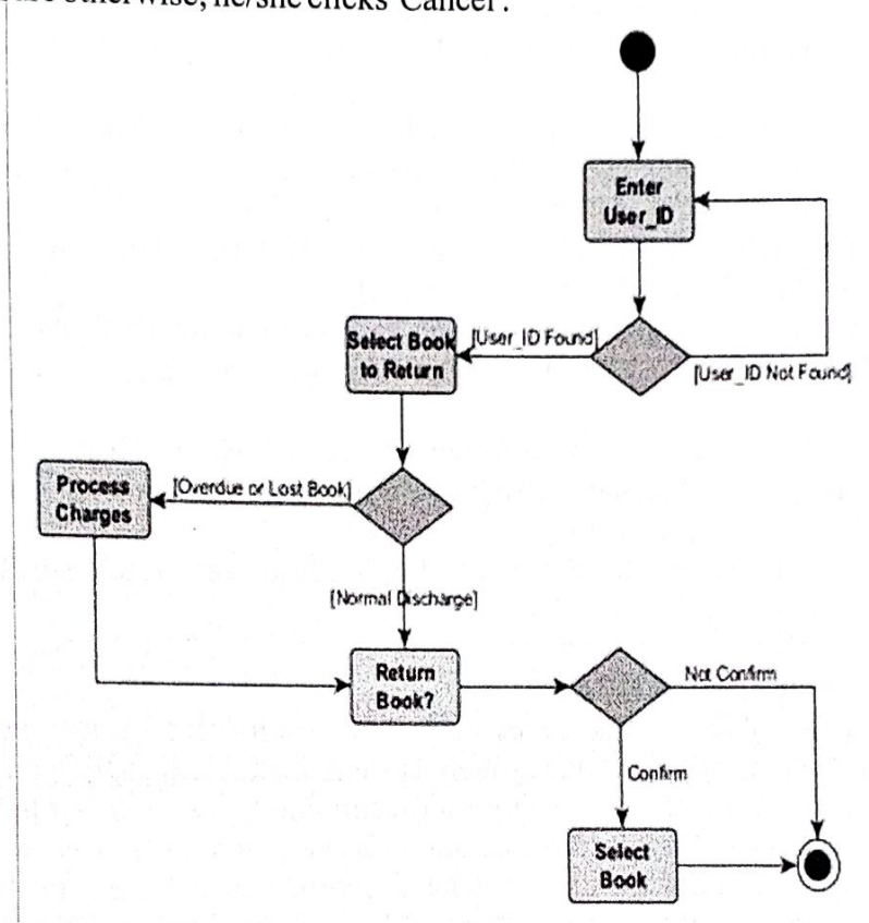
Figure 7: Activity Diagram for Book Discharging Process
