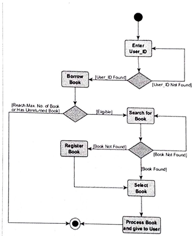
Figure 4: Activity Diagram for Local Book Borrowing Process
