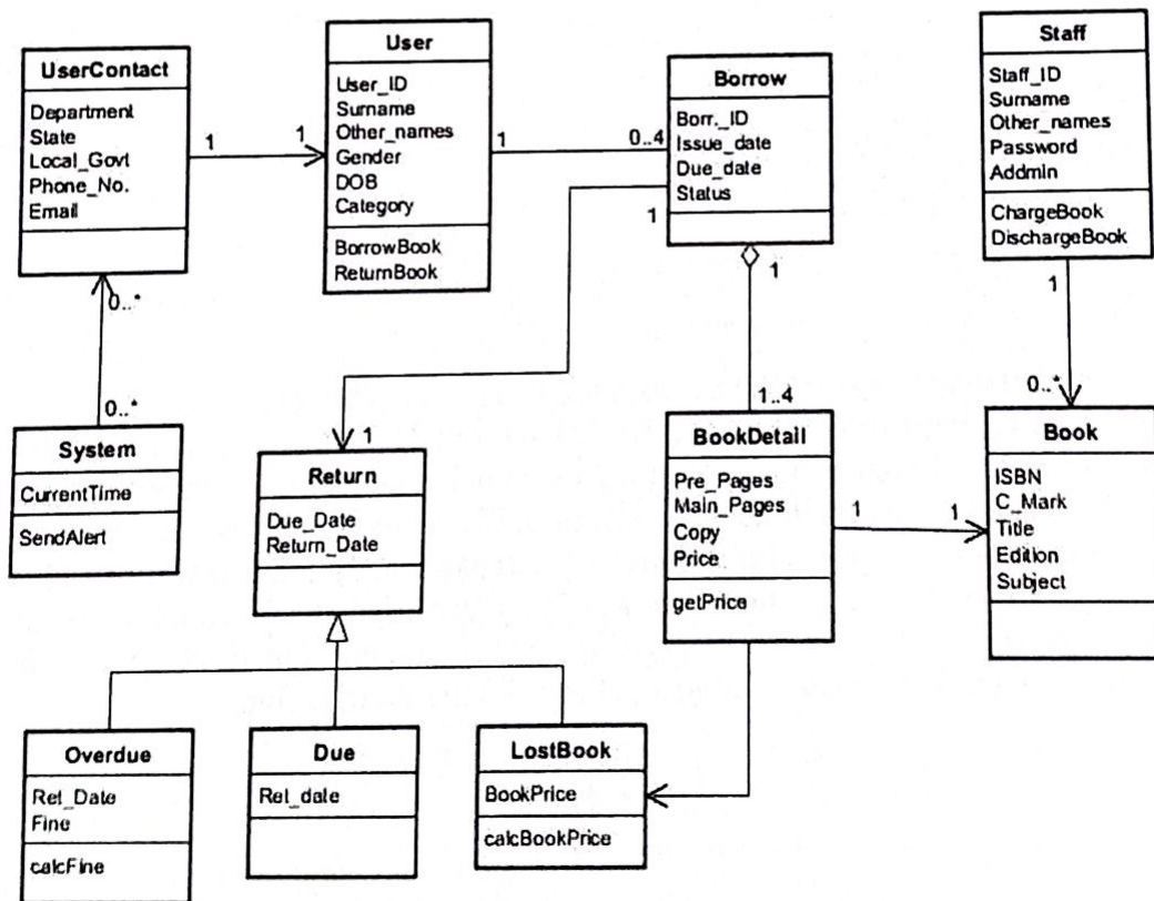
Figure 6: Class Diagram for Book Borrowing Process
