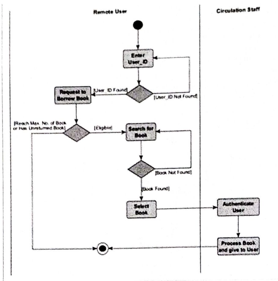
Figure 5: Activity Diagram for Remote Book Borrowing Process
