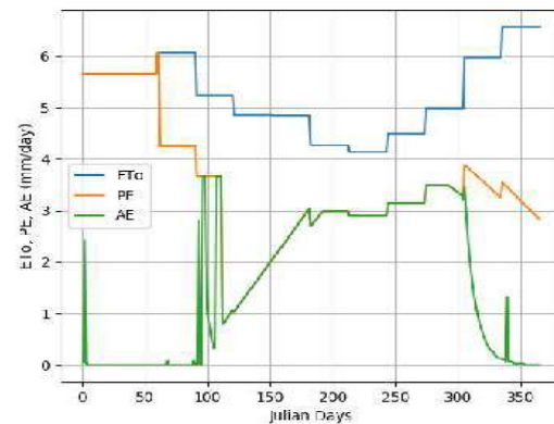
Figure 8: Relationship between ETo, PE and AE for 2008
