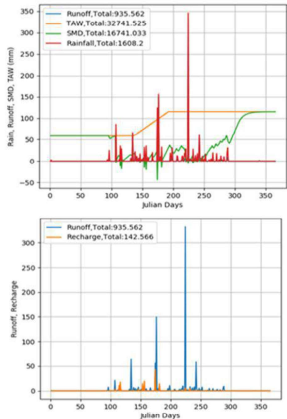
Figure 3: Modified Soil moisture balance components for Otukpo basin (2008)
