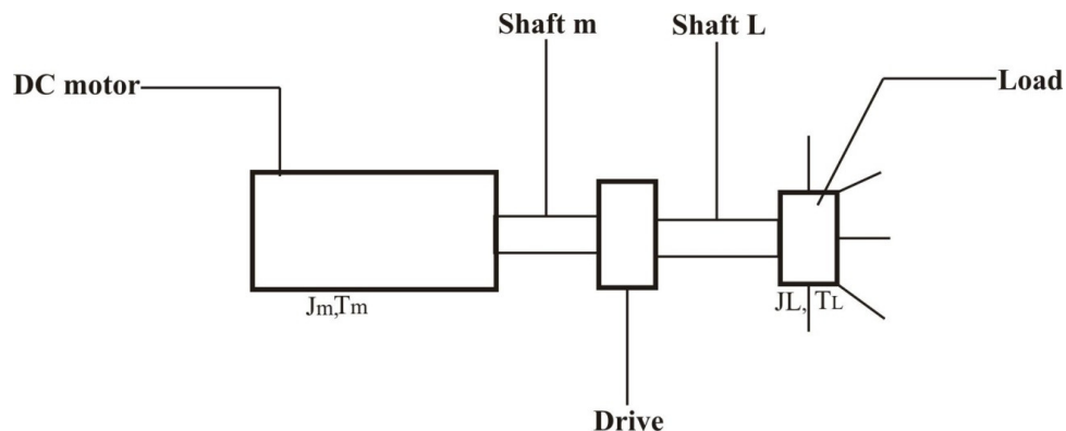
Figure 7: Electromechanical model of the motor and load
